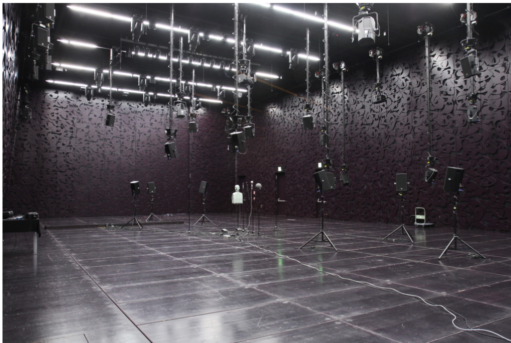
Figure 1. Motorised speaker rig and measurement setup at György Ligeti Hall at KUG Graz.
